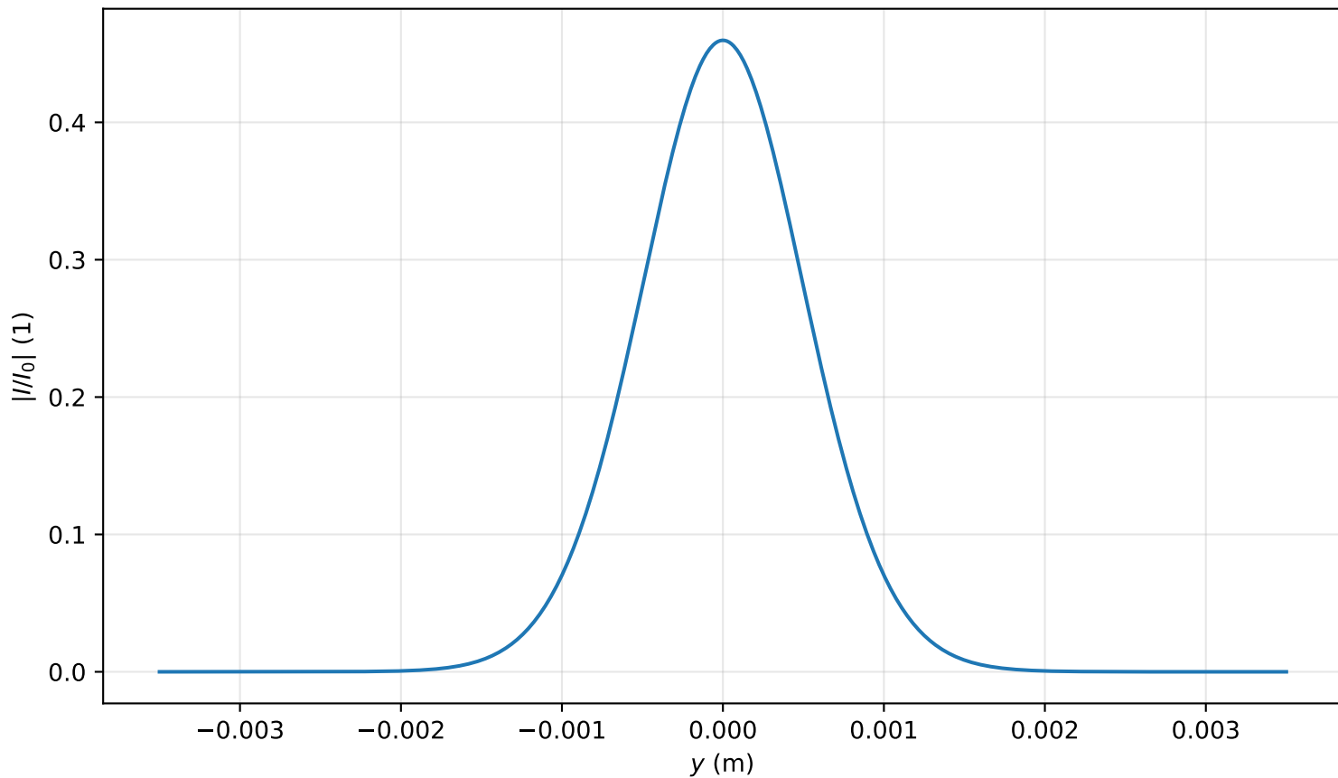
Intensity profile I(x = 0, y, z = 2.548)/I_0 , P_{in}=0.2P_{cr} , artificial time
